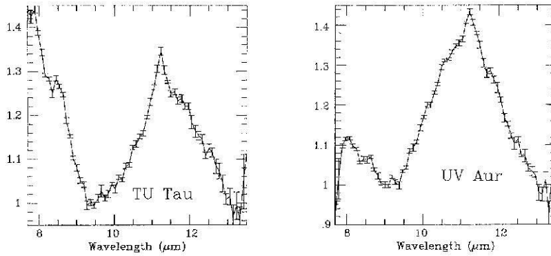
Figure 1. Normalised spectra of TU Tau and UV Aur
